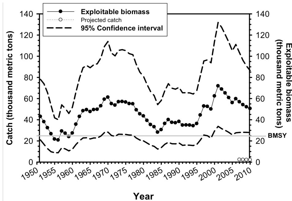
Figure 8. Exploitable biomass of swordfish in Sub-Area 2 (EPO) relative to exploitable biomass at maximum sustainable yield ( B_{MSY} ) from 1951 – 2006, and projected from 2007 – 2011 assuming the average harvest rate from 2004 – 2006.
