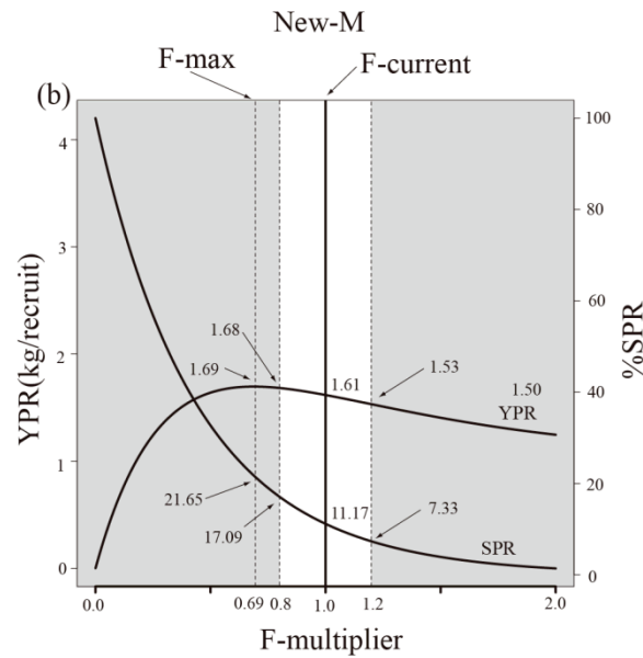
Figure 2. Yield per recruit curve and associated % spawners per recruit for Pacific bluefin tuna resulting from application of the new natural mortality (M) schedule as produced by the PBFWG at the 10-11 July 2009 working group meeting.
