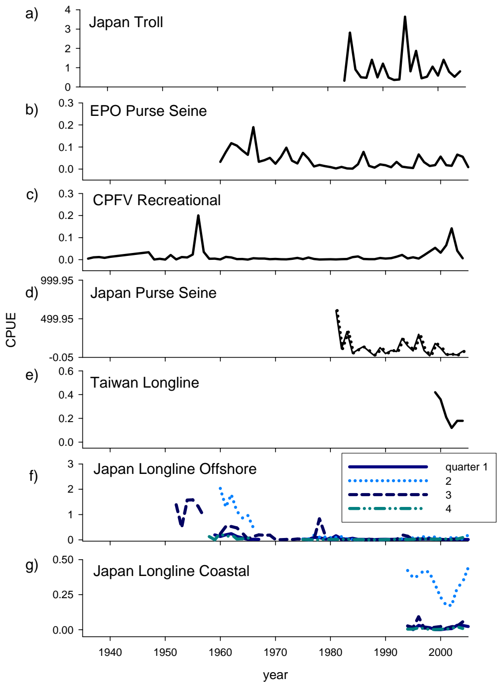
Figure 2. The estimated time series of CPUE from each data source. In d) the solid line depicts the annual index and the dotted line the quarterly index. In f) and g) the multiple plots represent quarterly indices.
